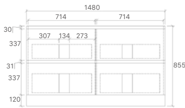
CORE-1500D Size:1480x455x855mm
