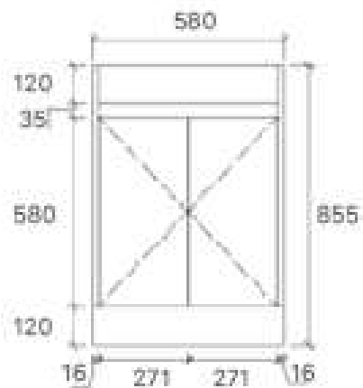
SY05-600 Size: 580x455x855mm
