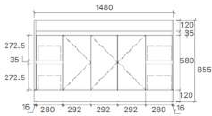
SY05-1500 Size: 1480x455x855mm
