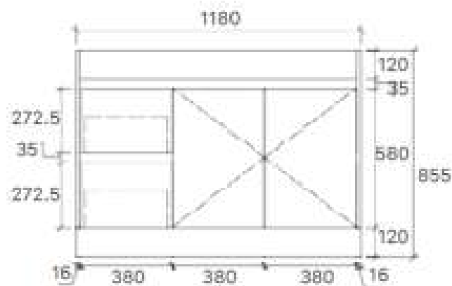
SY05-1200L Size: 1180x455x855mm
