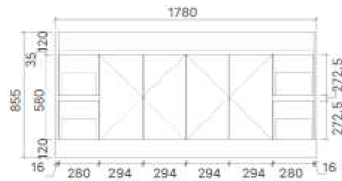
SY05-1800 Size: 1776x455x855mm
