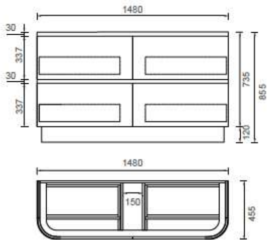
SK69-1500S Size: 1480x455x855Hmm
