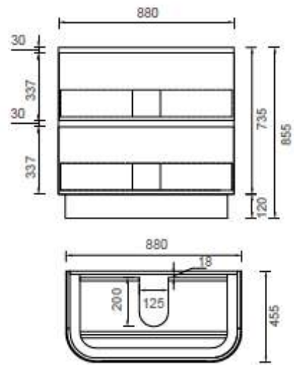
SK69-900 Size: 880x455x855Hmm
