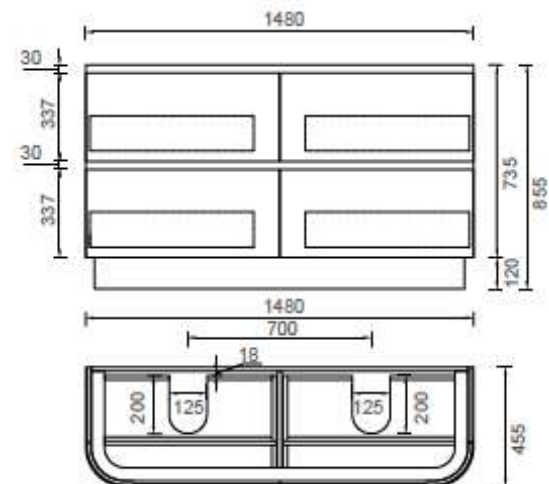
SK69-1500D Size: 1480x455x540Hmm
