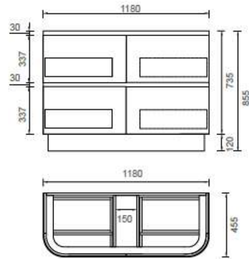
SK69-1200 Size: 1180x455x855Hmm
